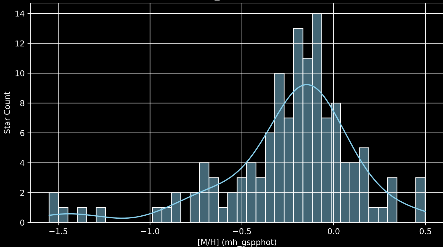
APOGEE DR17 Field: [044+47_MGA [M/H] (mh_gspphot) (n= 128)
