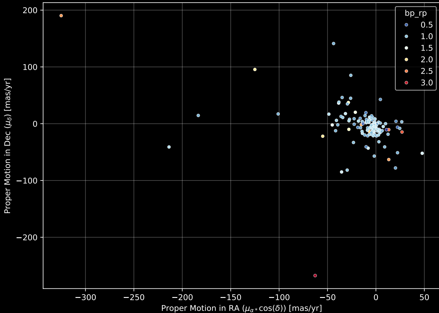
APOGEE DR17 Field: [044+47_MGA] Proper Motion Diagram (n= 130)
