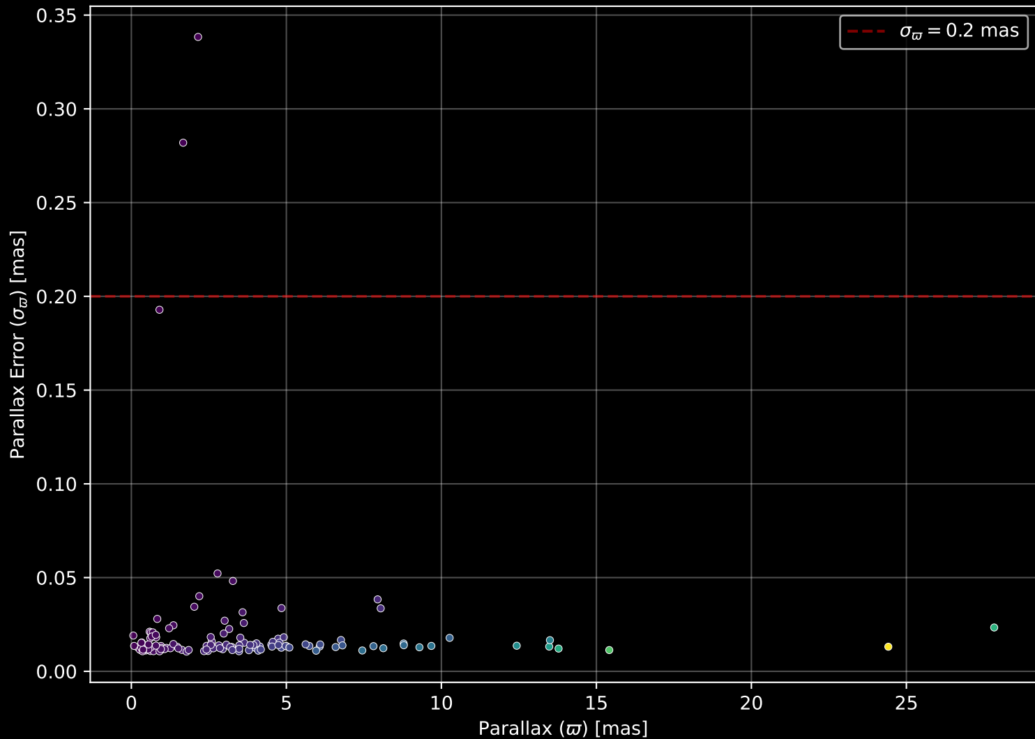
APOGEE DR17 Field: [044+47_MGA] Parallax Quality (n= 130)
