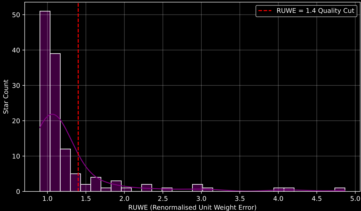
GAPOGEE DR17 Field [044+47_MGA] RUWE Distribution (n= 127)
