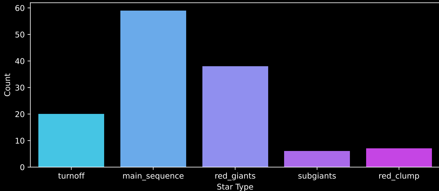
APOGEE DR17 Field: [044+47_MGA] Count plot of Star Type
